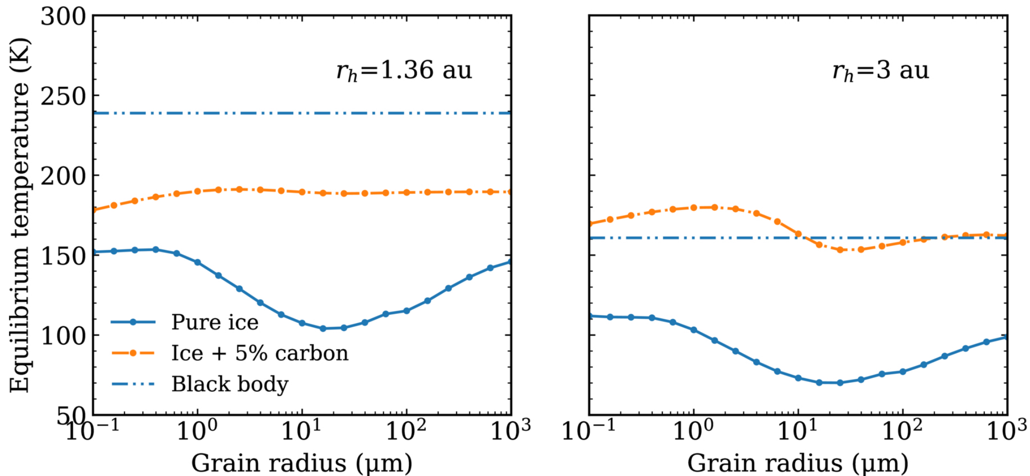
Figure C1. from Bin Liu et al 2026 Astrophys. J. Lett. 1008 doi:10.3847/2041-8213/ae9a89 https://dx.doi.org/10.3847/2041-8213/ae9a89 © 2026. The Author(s). Published by the American Astronomical Society.
