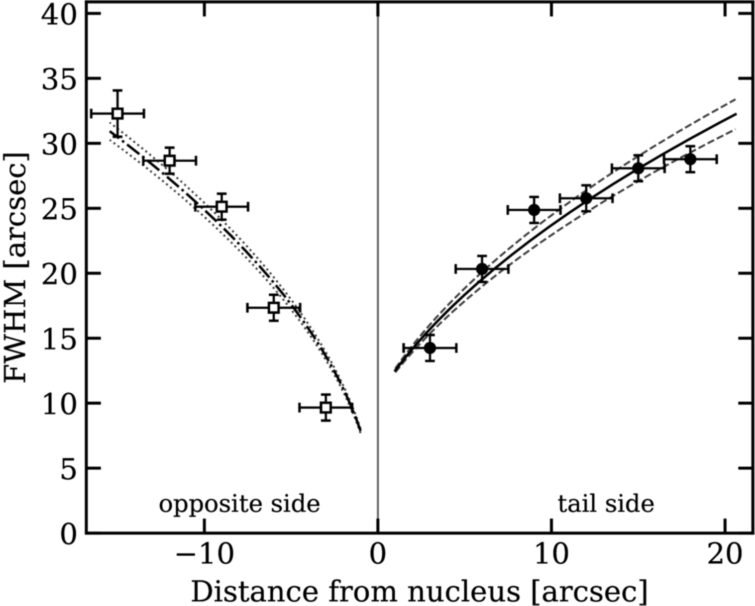
Figure A2. from Bin Liu et al 2026 Astrophys. J. Lett. 1008 doi:10.3847/2041-8213/ae9a89 https://dx.doi.org/10.3847/2041-8213/ae9a89 © 2026. The Author(s). Published by the American Astronomical Society.
