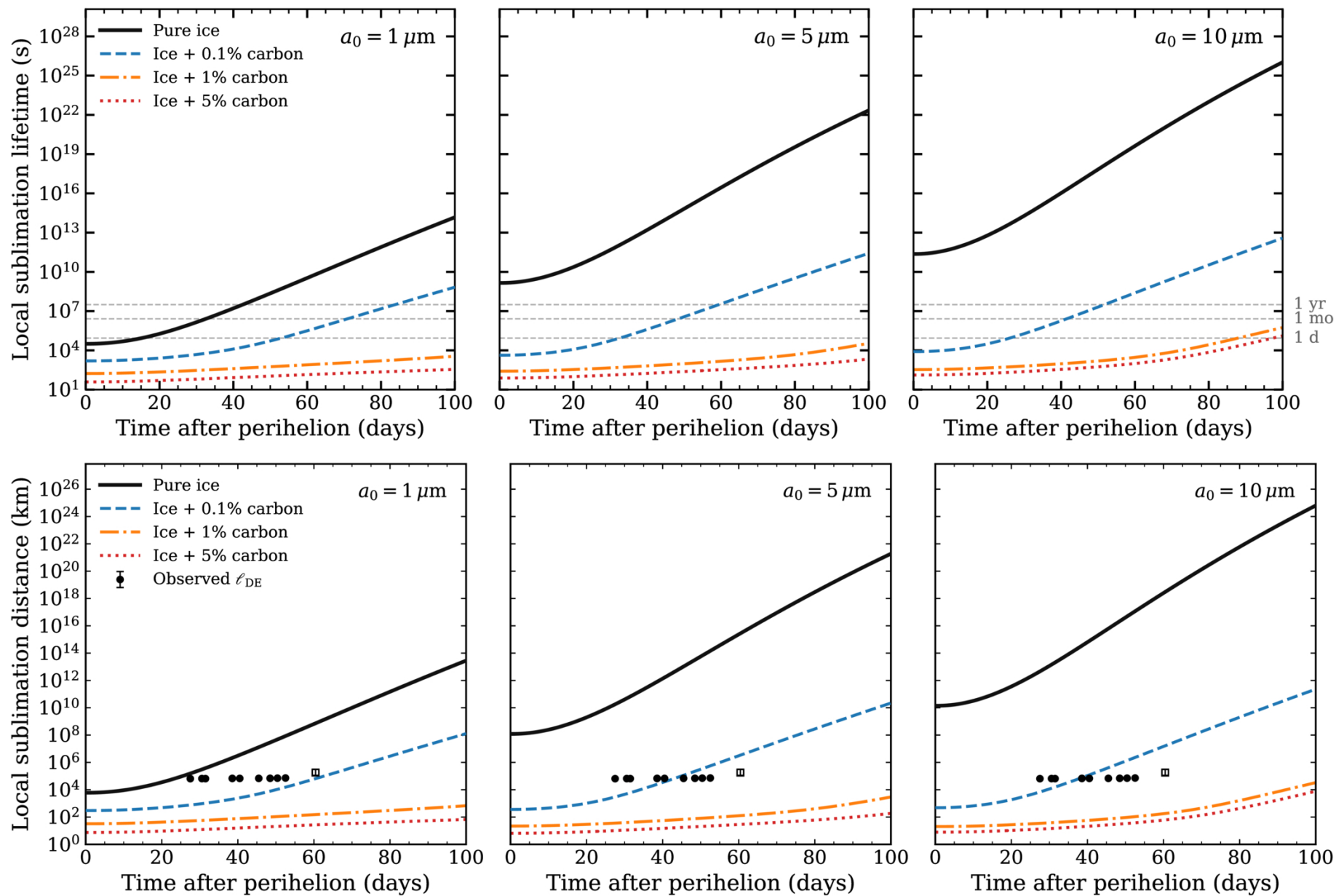
Figure 5. from Bin Liu et al 2026 Astrophys. J. Lett. 1008 doi:10.3847/2041-8213/ae9a89 https://dx.doi.org/10.3847/2041-8213/ae9a89 © 2026. The Author(s). Published by the American Astronomical Society.
