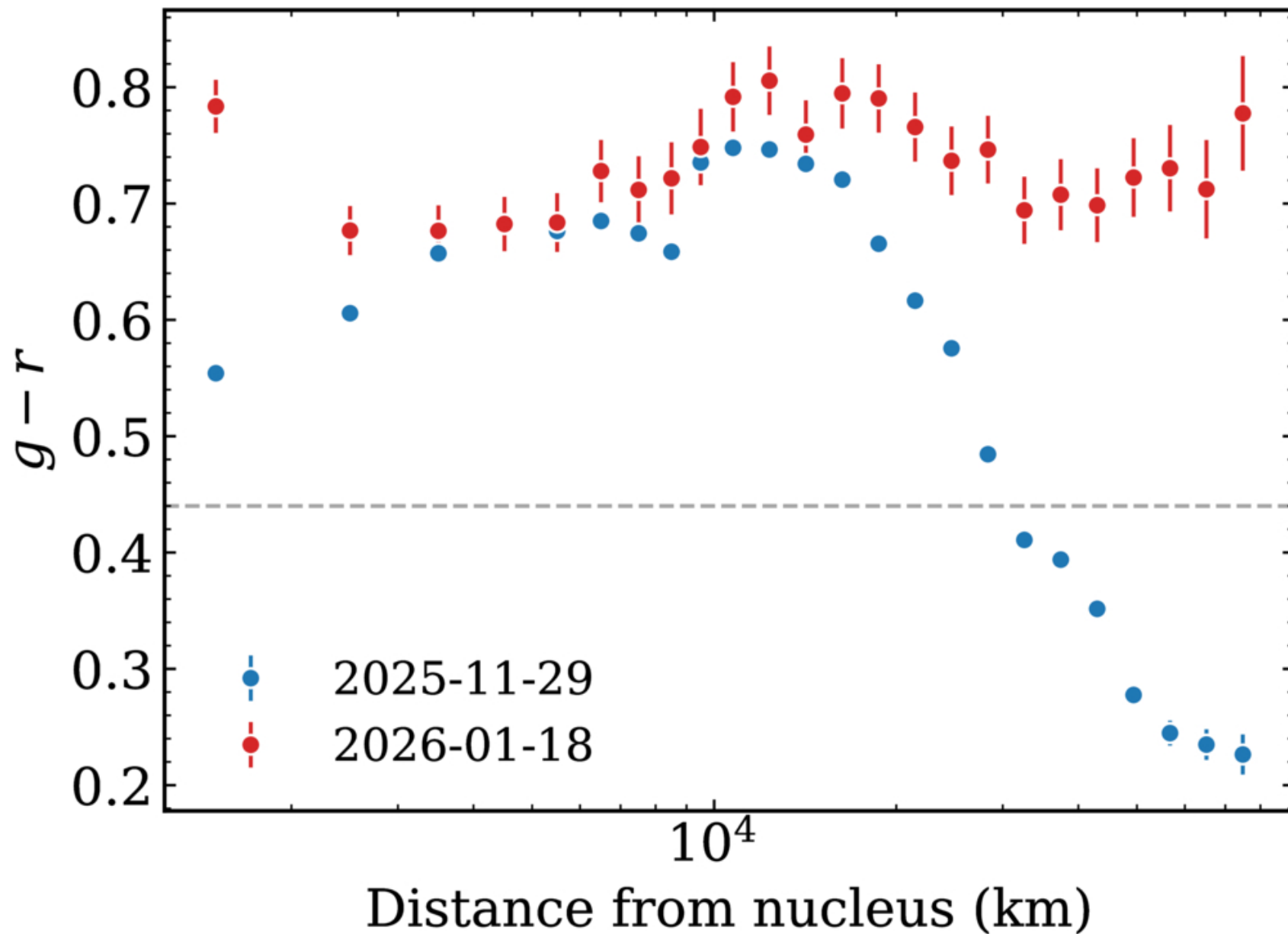
Figure 4. from Bin Liu et al 2026 Astrophys. J. Lett. 1008 doi:10.3847/2041-8213/ae9a89 https://dx.doi.org/10.3847/2041-8213/ae9a89 © 2026. The Author(s). Published by the American Astronomical Society.
