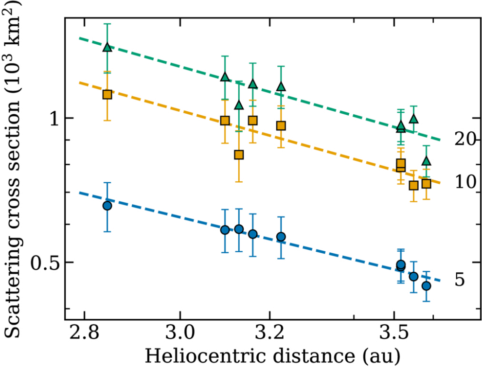
Figure 3. from Bin Liu et al 2026 Astrophys. J. Lett. 1008 doi:10.3847/2041-8213/ae9a89 https://dx.doi.org/10.3847/2041-8213/ae9a89 © 2026. The Author(s). Published by the American Astronomical Society.
