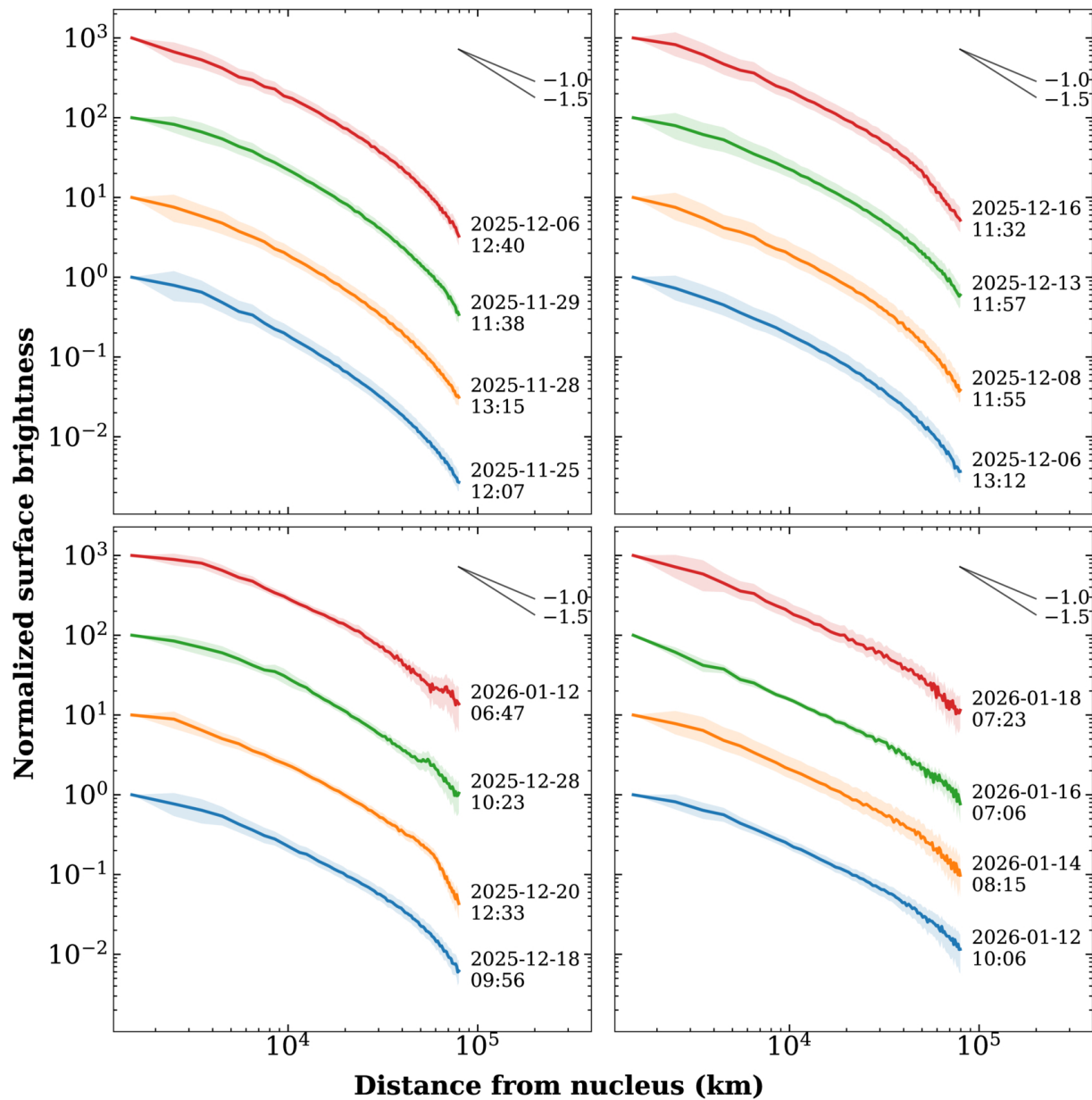
Figure 2. from Bin Liu et al 2026 Astrophys. J. Lett. 1008 doi:10.3847/2041-8213/ae9a89 https://dx.doi.org/10.3847/2041-8213/ae9a89 © 2026. The Author(s). Published by the American Astronomical Society.
