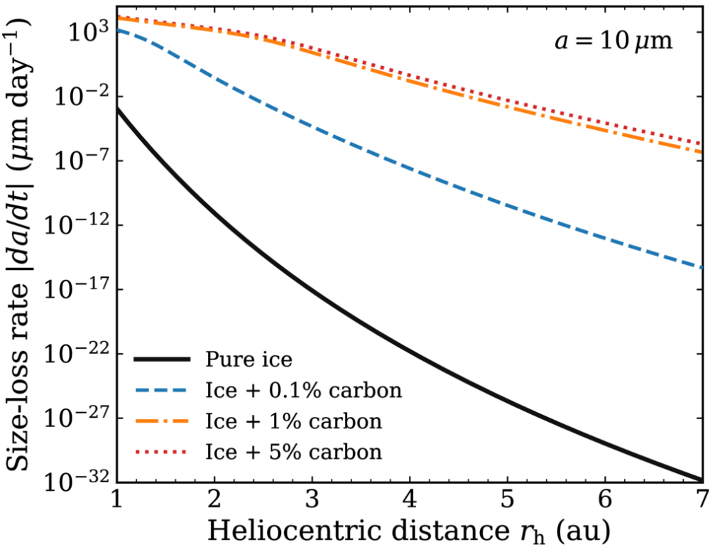
Figure C2. from Bin Liu et al 2026 Astrophys. J. Lett. 1008 doi:10.3847/2041-8213/ae9a89 https://dx.doi.org/10.3847/2041-8213/ae9a89 © 2026. The Author(s). Published by the American Astronomical Society.
