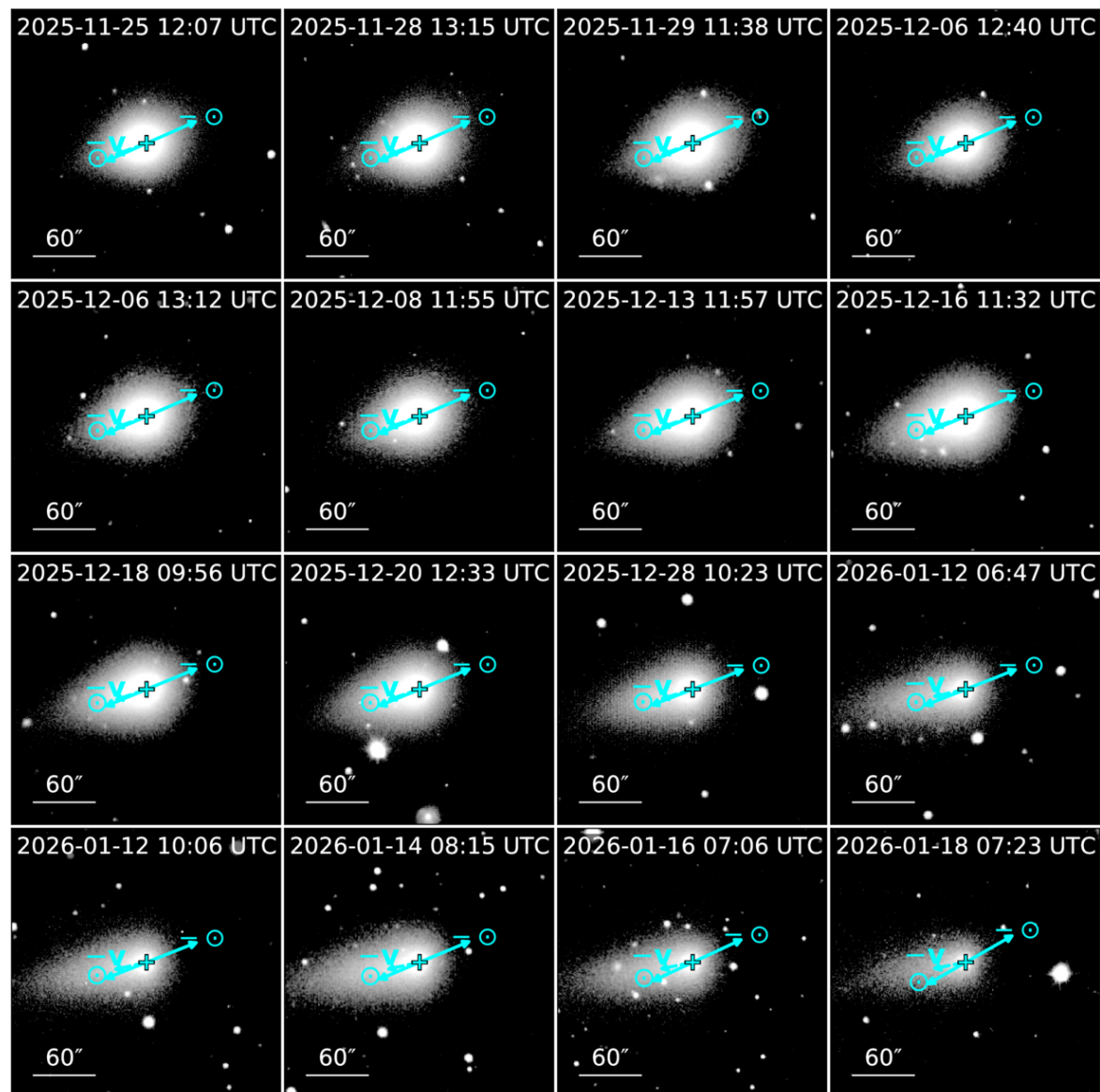
(b) Post-perihelion images.
