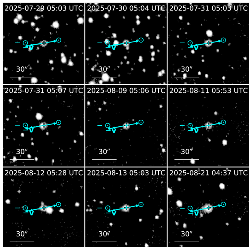
(a) Pre-perihelion images.
