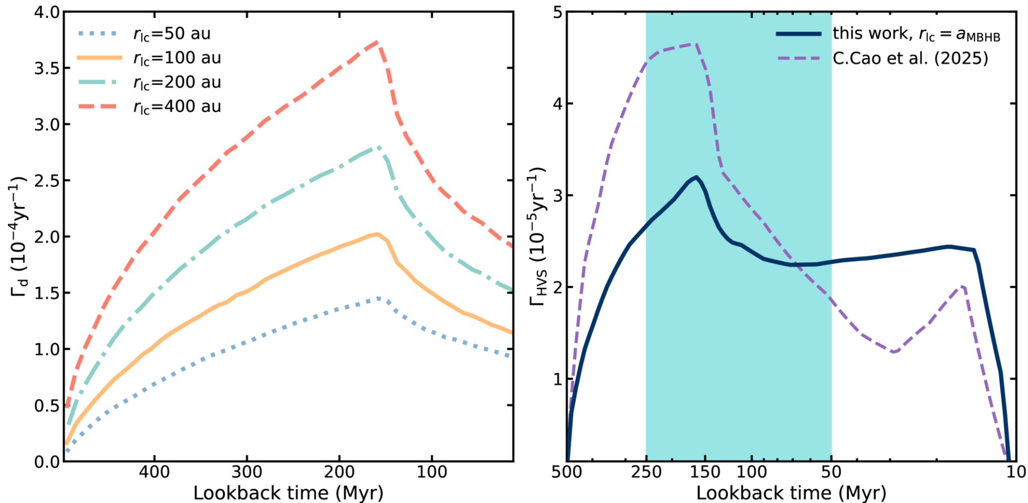
Figure 4. from Chunyang Cao et al 2026 Astrophys. J. Lett. 1009 doi:10.3847/2041-8213/ae9a72 https://dx.doi.org/10.3847/2041-8213/ae9a72 © 2026. The Author(s). Published by the American Astronomical Society.
