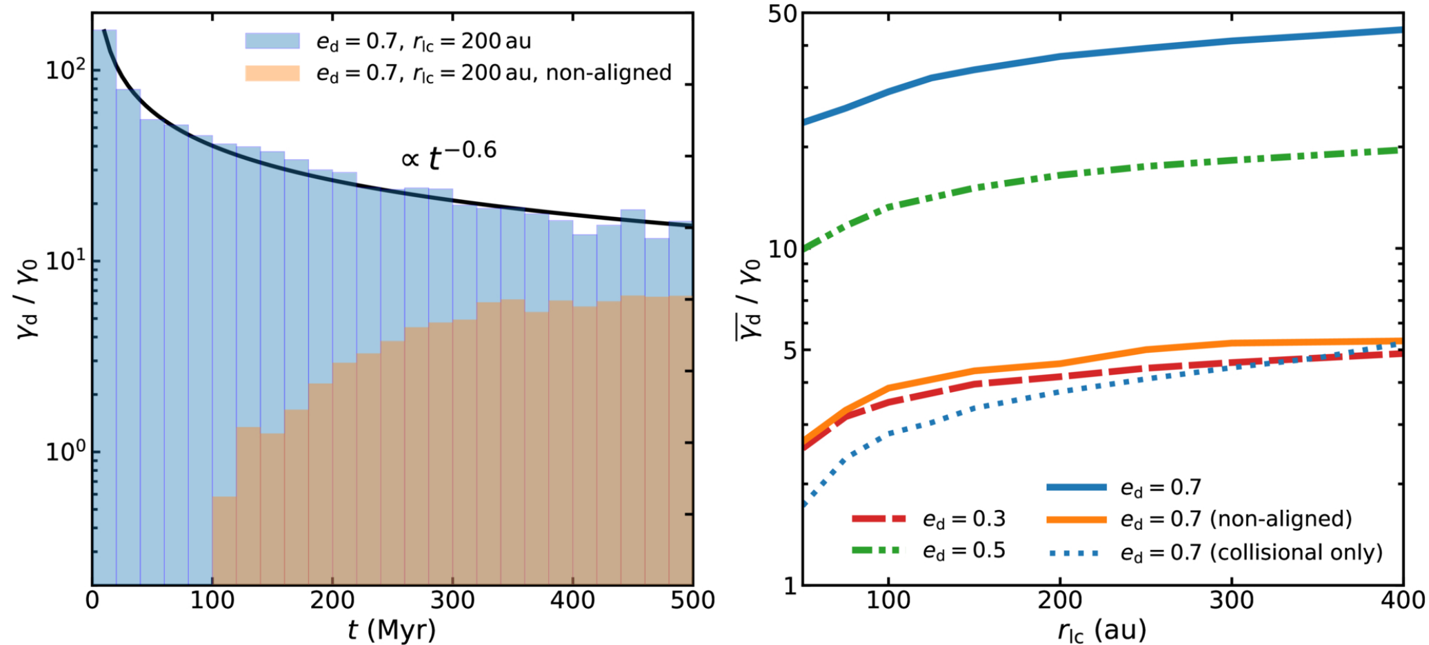
Figure 3. from Chunyang Cao et al 2026 Astrophys. J. Lett. 1009 doi:10.3847/2041-8213/ae9a72 https://dx.doi.org/10.3847/2041-8213/ae9a72 © 2026. The Author(s). Published by the American Astronomical Society.
