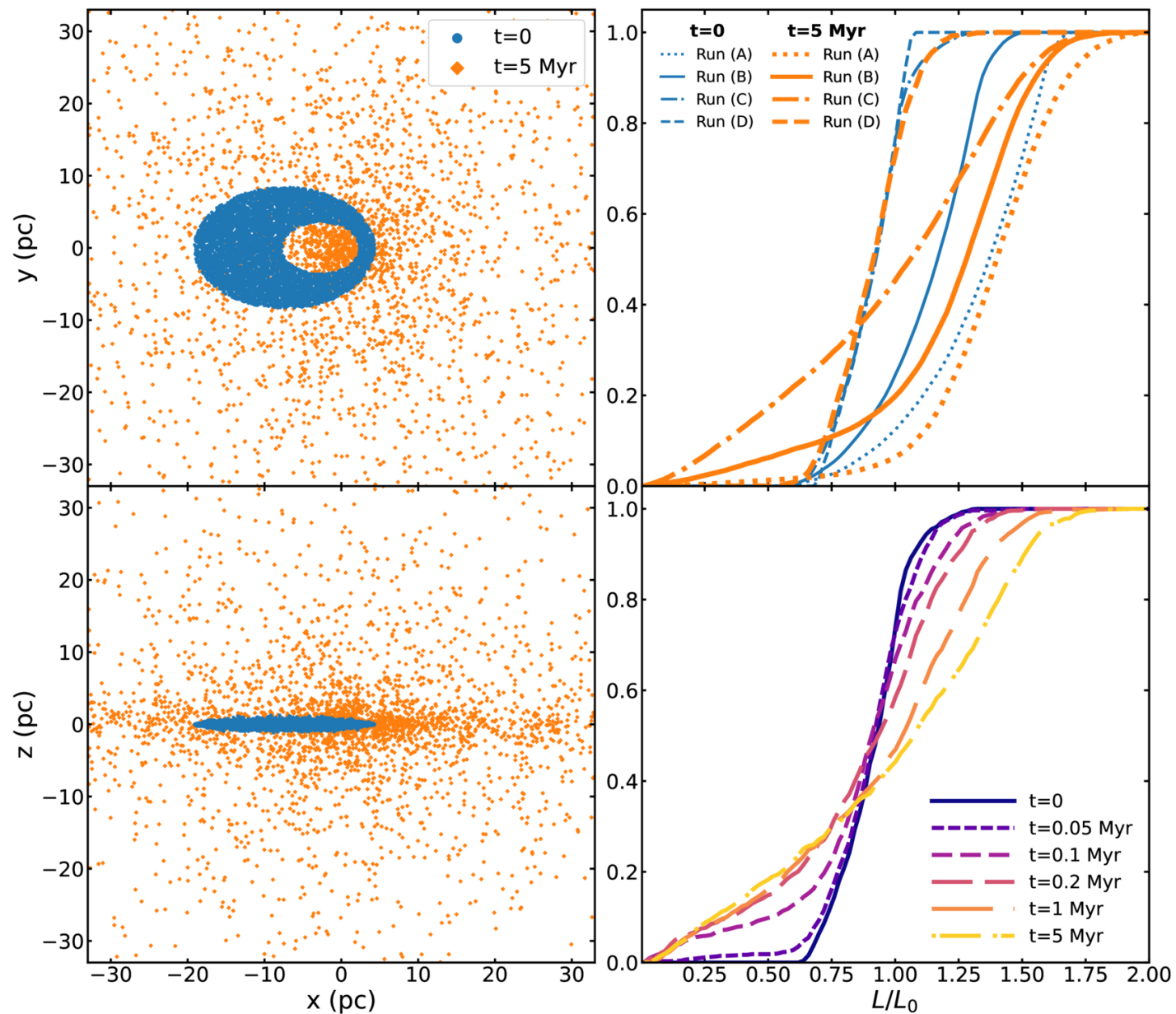
Figure 1. from Chunyang Cao et al 2026 Astrophys. J. Lett. 1009 doi:10.3847/2041-8213/ae9a72 https://dx.doi.org/10.3847/2041-8213/ae9a72 © 2026. The Author(s). Published by the American Astronomical Society.
