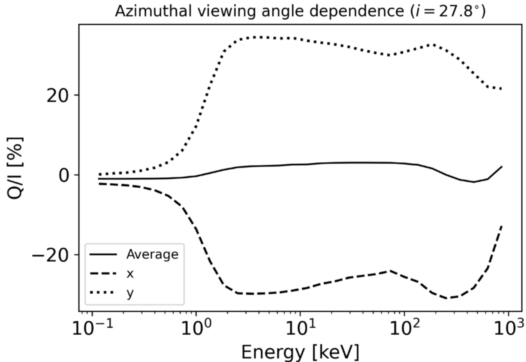
Figure 8. from John Groger et al 2026 Astrophys. J. Lett. 1008 doi:10.3847/2041-8213/ae99de https://dx.doi.org/10.3847/2041-8213/ae99de © 2026. The Author(s). Published by the American Astronomical Society.
