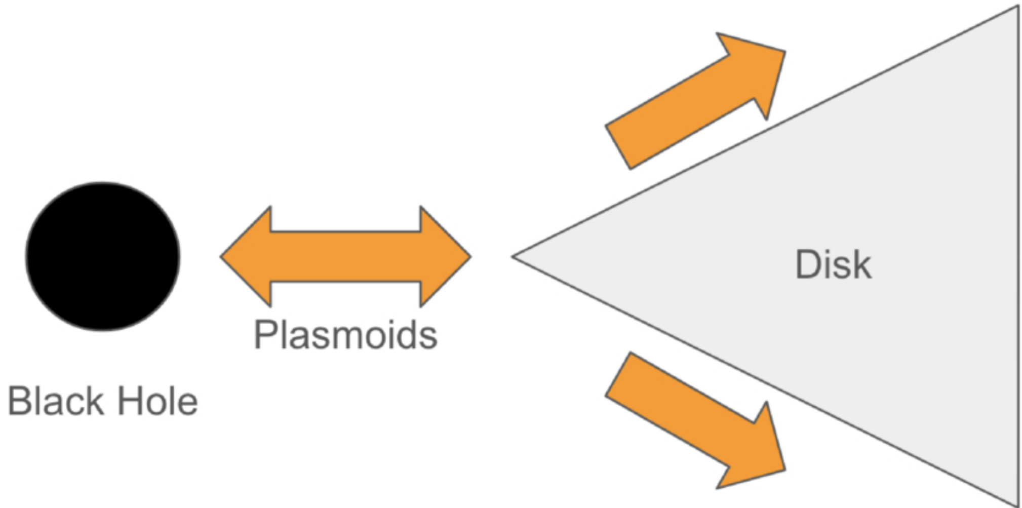
Figure 7. from John Groger et al 2026 Astrophys. J. Lett. 1008 doi:10.3847/2041-8213/ae99de https://dx.doi.org/10.3847/2041-8213/ae99de © 2026. The Author(s). Published by the American Astronomical Society.
