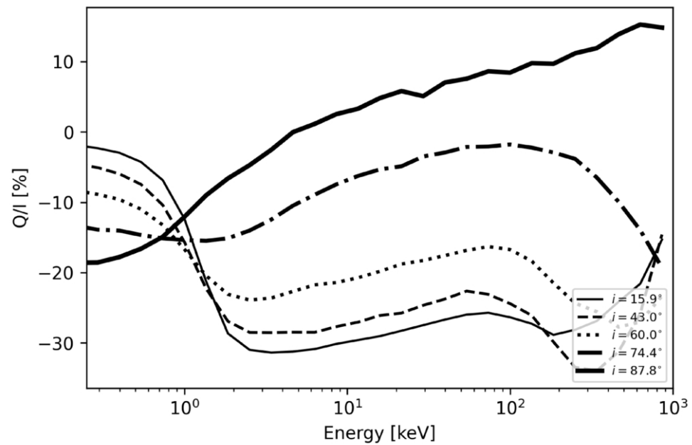
Figure 6. from John Groger et al 2026 Astrophys. J. Lett. 1008 doi:10.3847/2041-8213/ae99de https://dx.doi.org/10.3847/2041-8213/ae99de © 2026. The Author(s). Published by the American Astronomical Society.
