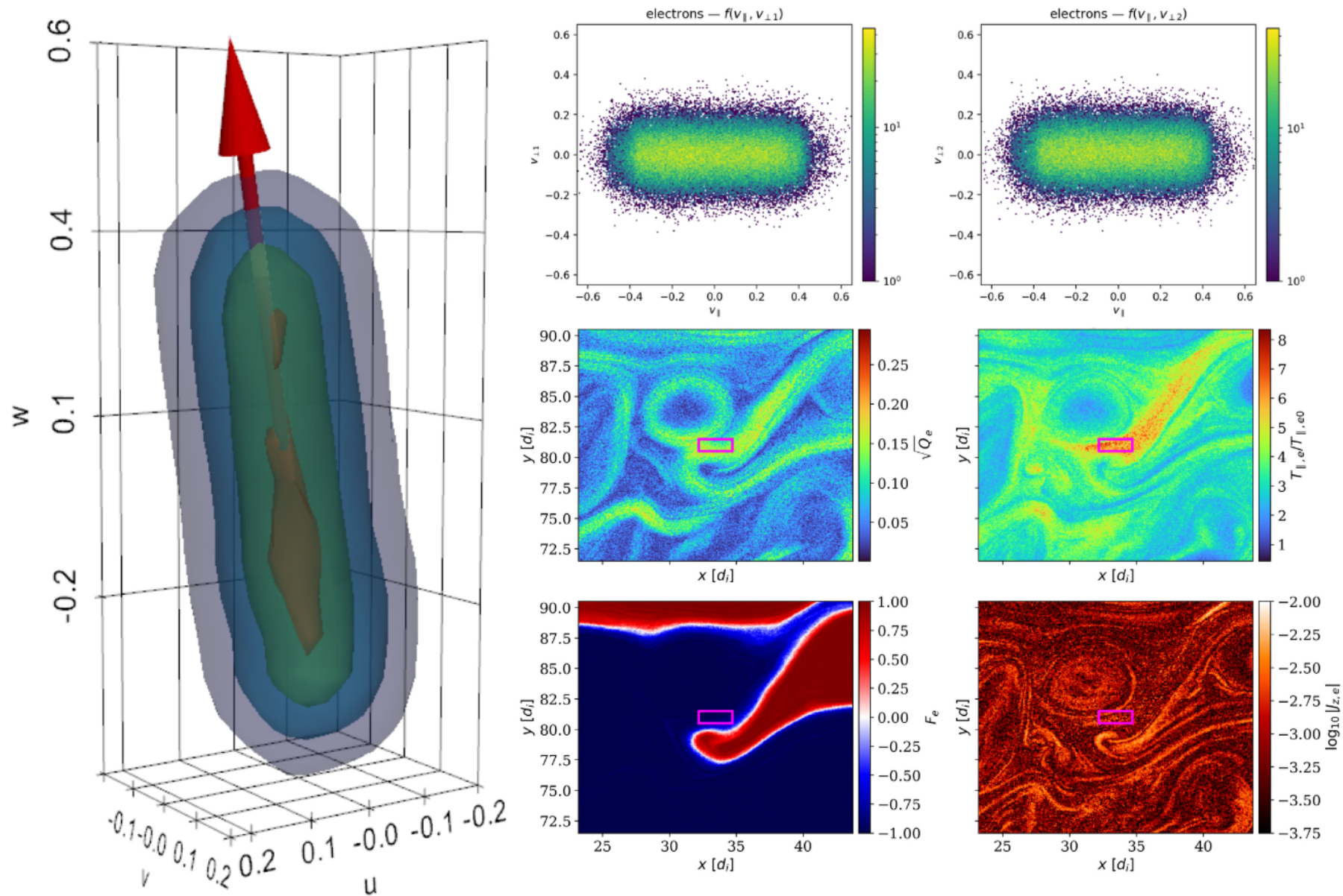
Figure C1. from Silvia Ferro et al 2026 Astrophys. J. Lett. 1008 doi:10.3847/2041-8213/ae99ca https://dx.doi.org/10.3847/2041-8213/ae99ca © 2026. The Author(s). Published by the American Astronomical Society.
