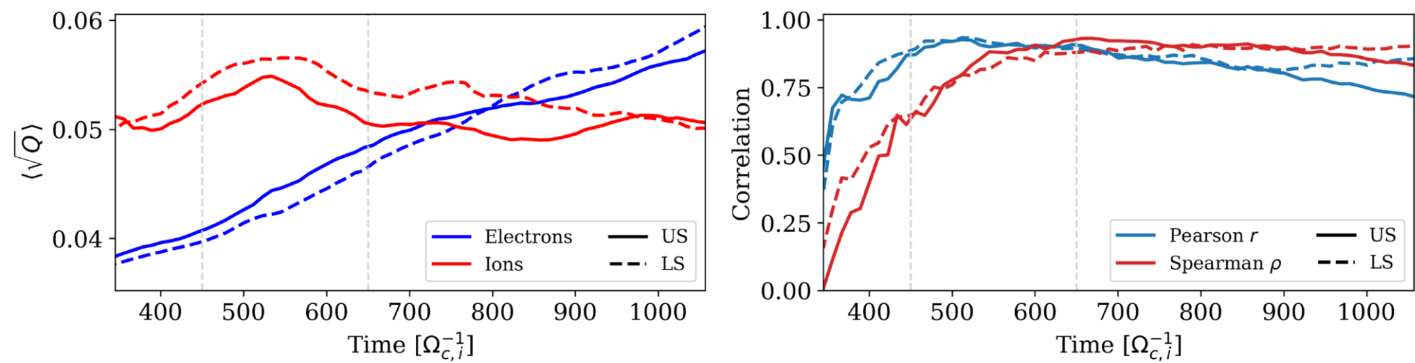
Figure B1. from Silvia Ferro et al 2026 Astrophys. J. Lett. 1008 doi:10.3847/2041-8213/ae99ca https://dx.doi.org/10.3847/2041-8213/ae99ca © 2026. The Author(s). Published by the American Astronomical Society.
