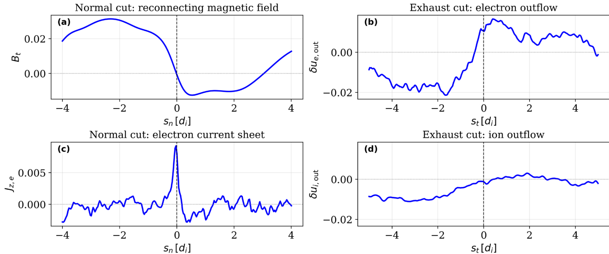
Figure A2. from Silvia Ferro et al 2026 Astrophys. J. Lett. 1008 doi:10.3847/2041-8213/ae99ca https://dx.doi.org/10.3847/2041-8213/ae99ca © 2026. The Author(s). Published by the American Astronomical Society.
