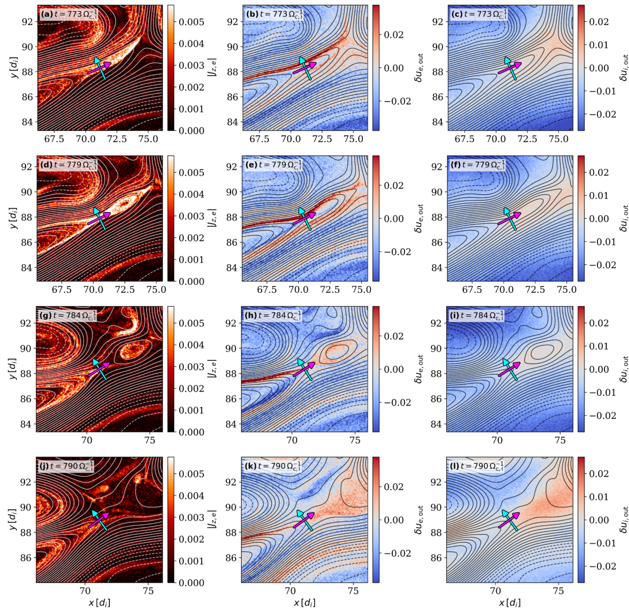
Figure A1. from Silvia Ferro et al 2026 Astrophys. J. Lett. 1008 doi:10.3847/2041-8213/ae99ca https://dx.doi.org/10.3847/2041-8213/ae99ca © 2026. The Author(s). Published by the American Astronomical Society.
