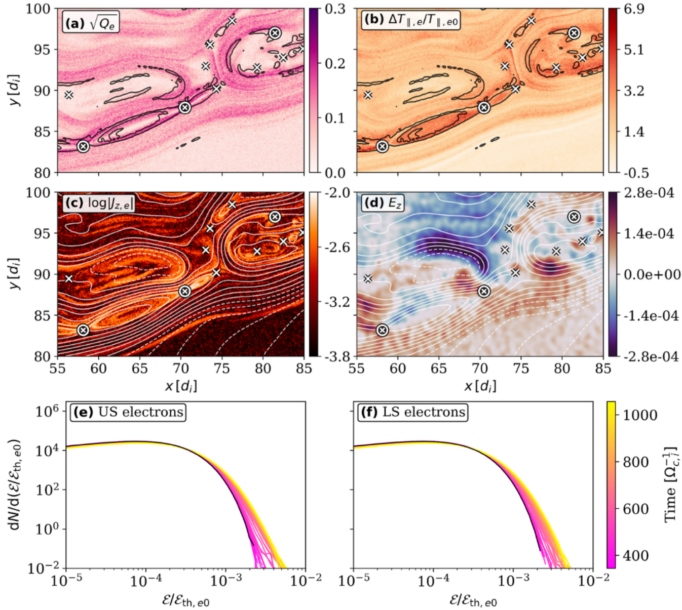
Figure 5. from Silvia Ferro et al 2026 Astrophys. J. Lett. 1008 doi:10.3847/2041-8213/ae99ca https://dx.doi.org/10.3847/2041-8213/ae99ca © 2026. The Author(s). Published by the American Astronomical Society.
