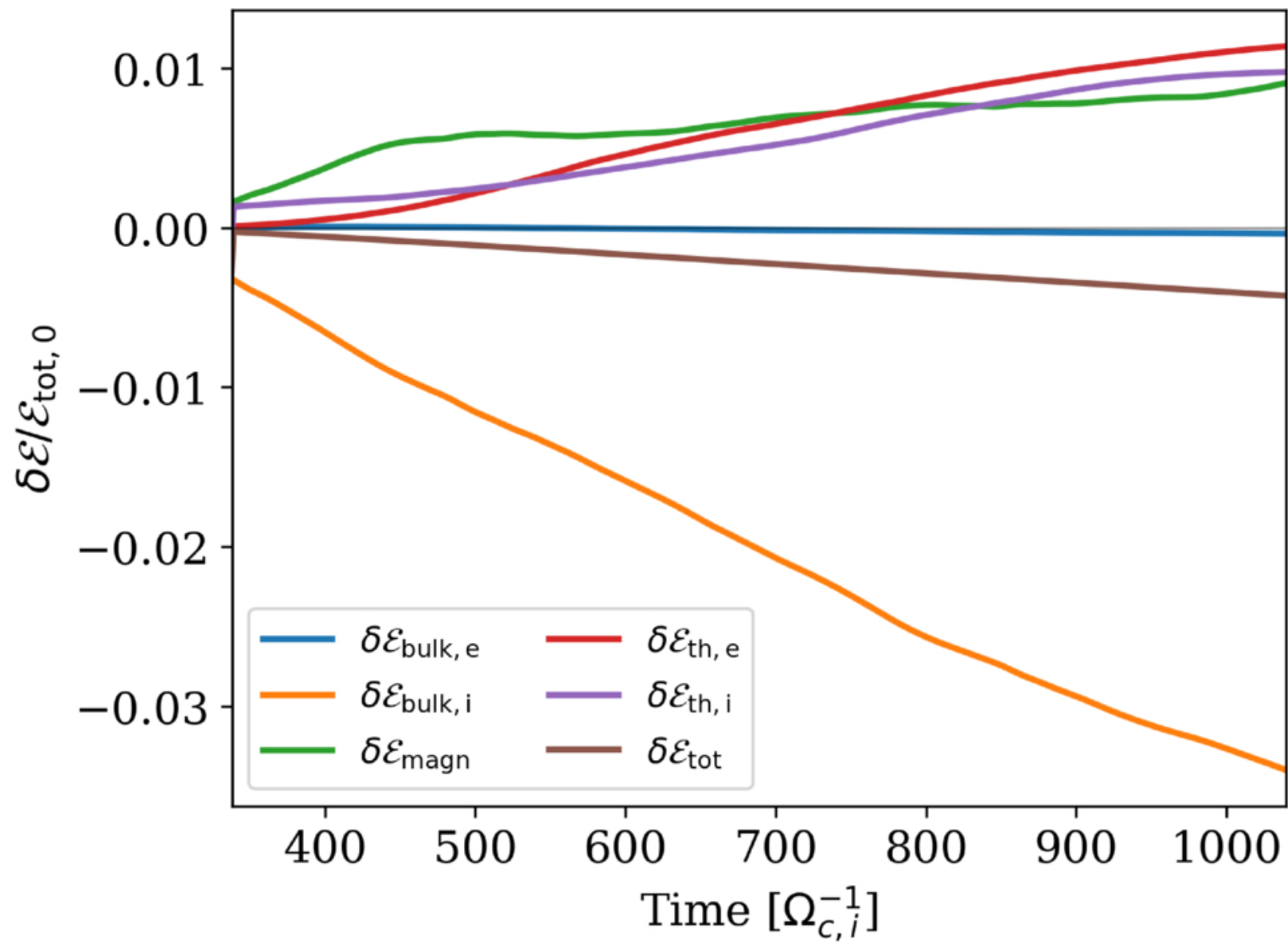
Figure 2. from Silvia Ferro et al 2026 Astrophys. J. Lett. 1008 doi:10.3847/2041-8213/ae99ca https://dx.doi.org/10.3847/2041-8213/ae99ca © 2026. The Author(s). Published by the American Astronomical Society.
