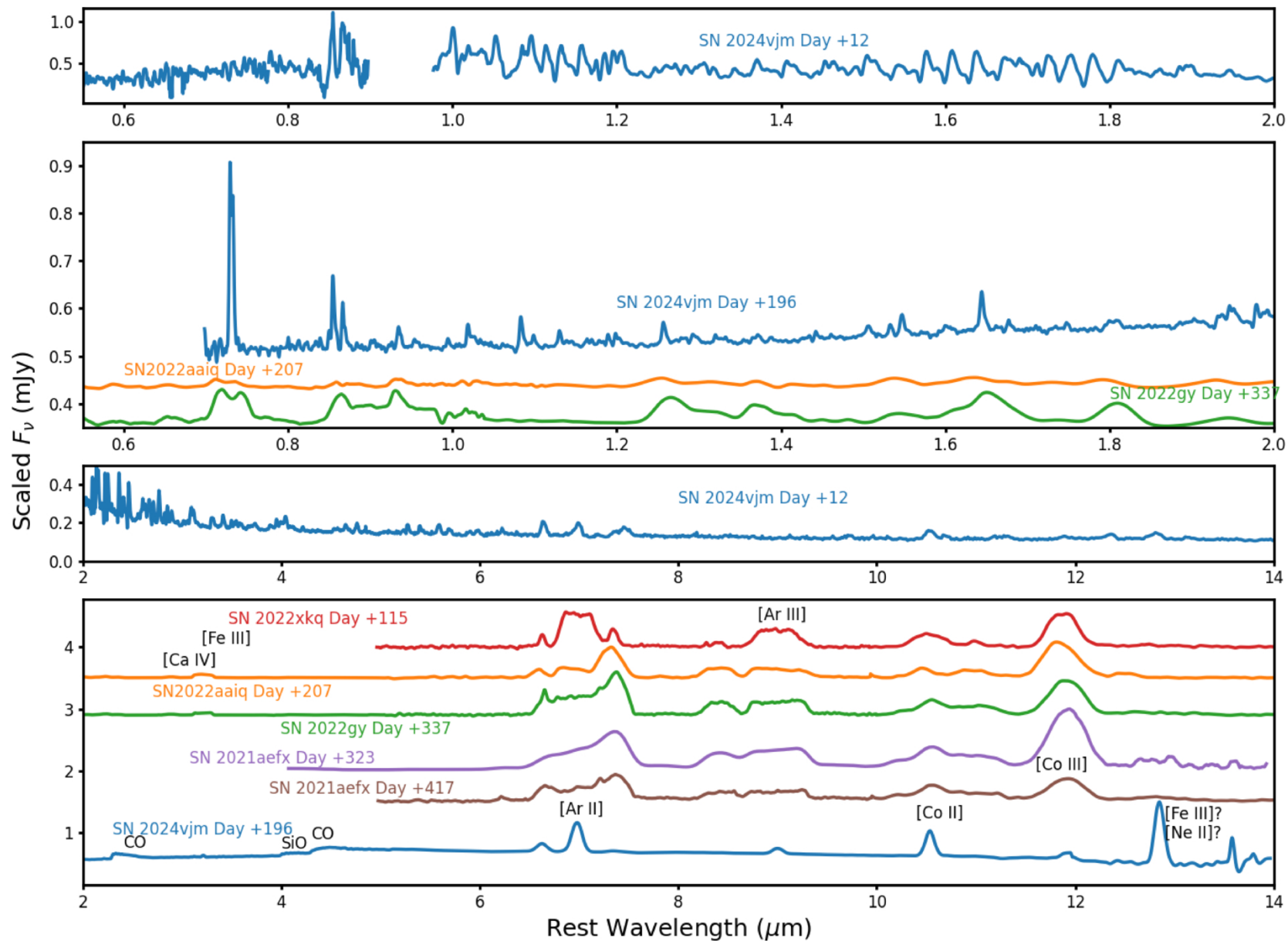
Figure 5. from E. Baron et al 2026 Astrophys. J. Lett. 1008 doi:10.3847/2041-8213/ae99c9 https://dx.doi.org/10.3847/2041-8213/ae99c9 © 2026. The Author(s). Published by the American Astronomical Society.
