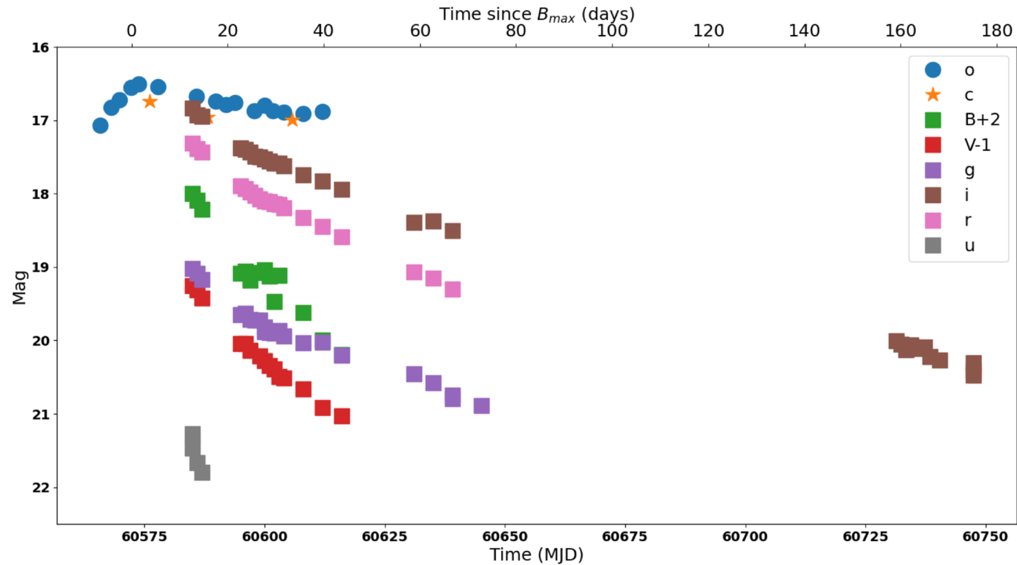
Figure 2. from E. Baron et al 2026 Astrophys. J. Lett. 1008 doi:10.3847/2041-8213/ae99c9 https://dx.doi.org/10.3847/2041-8213/ae99c9 © 2026. The Author(s). Published by the American Astronomical Society.
