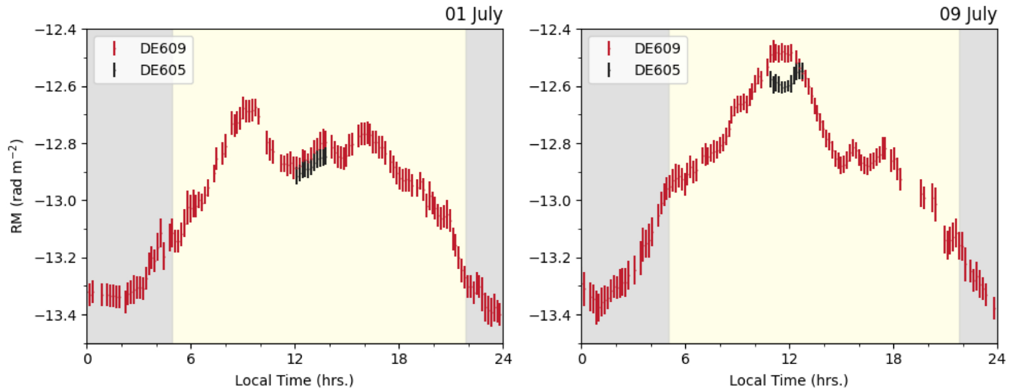
Figure 3. from Yanqing Cai et al 2026 Astrophys. J. Lett. 1008 doi:10.3847/2041-8213/ae993d https://dx.doi.org/10.3847/2041-8213/ae993d © 2026. The Author(s). Published by the American Astronomical Society.
