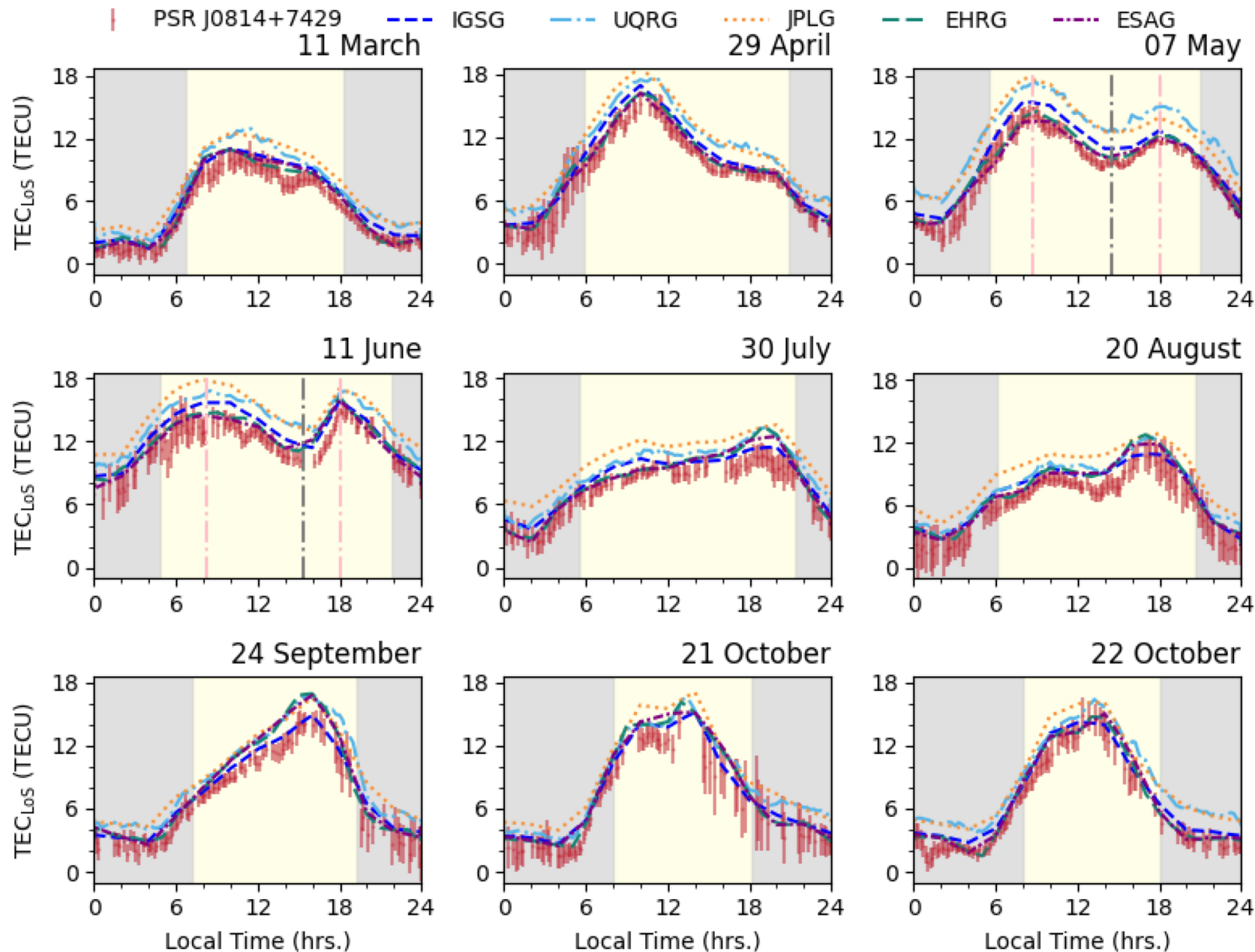
Figure 2. from Yanqing Cai et al 2026 Astrophys. J. Lett. 1008 doi:10.3847/2041-8213/ae993d https://dx.doi.org/10.3847/2041-8213/ae993d © 2026. The Author(s). Published by the American Astronomical Society.
