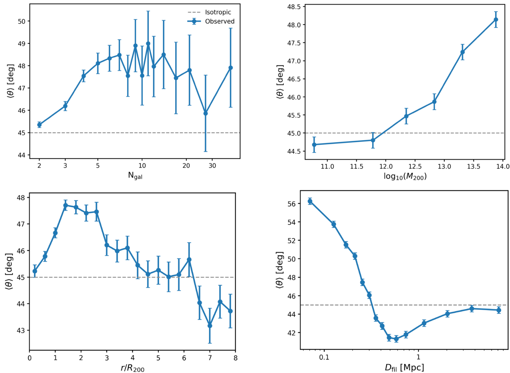
Figure 2. from Peng Wang et al 2026 Astrophys. J. Lett. 1008 doi:10.3847/2041-8213/ae9935 https://dx.doi.org/10.3847/2041-8213/ae9935 © 2026. The Author(s). Published by the American Astronomical Society.
