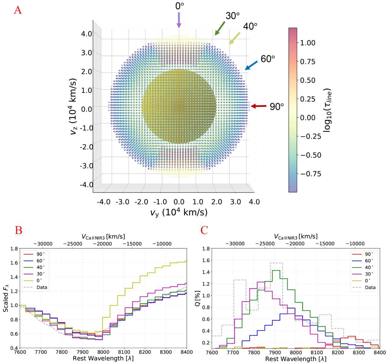
Figure A3. from Xudong Wen et al 2026 Astrophys. J. Lett. 1008 doi:10.3847/2041-8213/ae990c https://dx.doi.org/10.3847/2041-8213/ae990c © 2026. The Author(s). Published by the American Astronomical Society.
