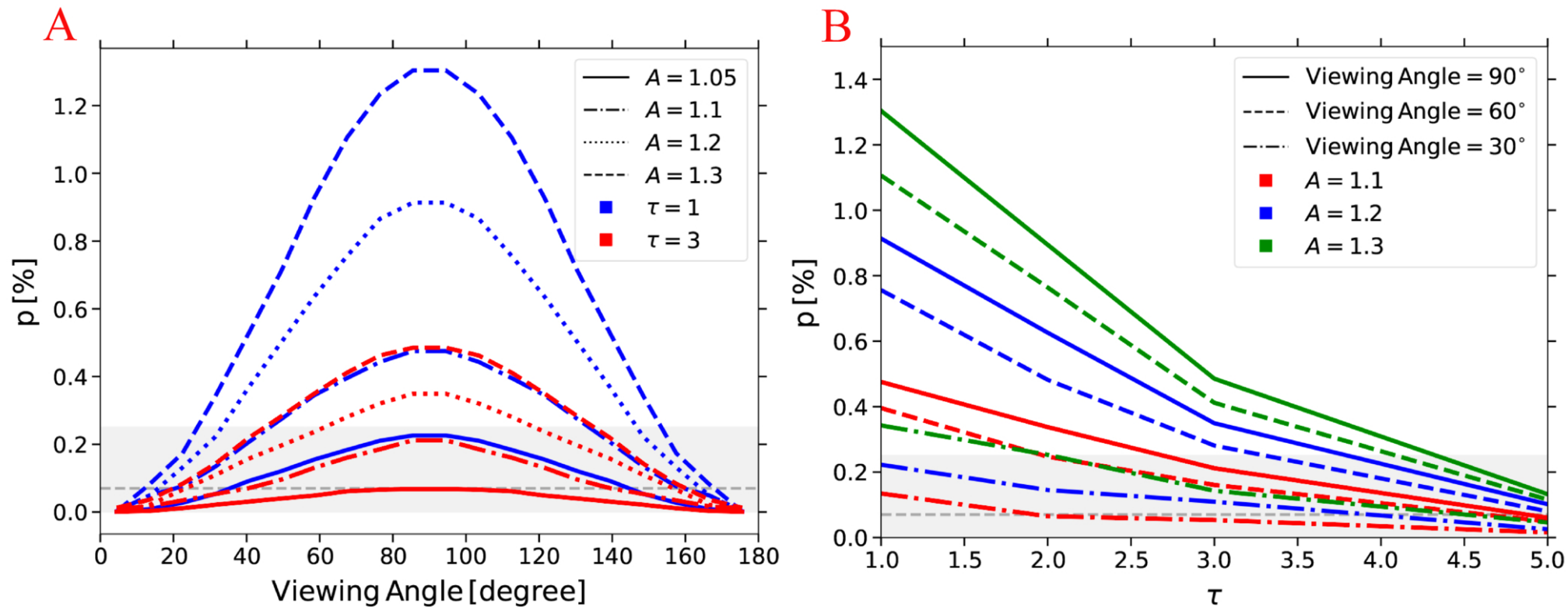
Figure A2. from Xudong Wen et al 2026 Astrophys. J. Lett. 1008 doi:10.3847/2041-8213/ae990c https://dx.doi.org/10.3847/2041-8213/ae990c © 2026. The Author(s). Published by the American Astronomical Society.
