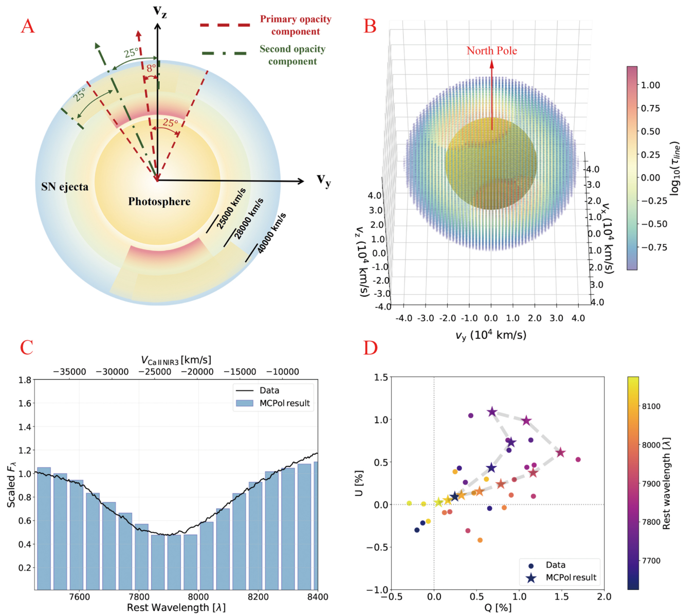
Figure 3. from Xudong Wen et al 2026 Astrophys. J. Lett. 1008 doi:10.3847/2041-8213/ae990c https://dx.doi.org/10.3847/2041-8213/ae990c © 2026. The Author(s). Published by the American Astronomical Society.
