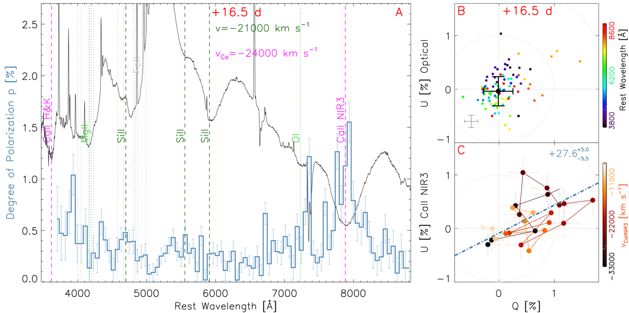
Figure 2. from Xudong Wen et al 2026 Astrophys. J. Lett. 1008 doi:10.3847/2041-8213/ae990c https://dx.doi.org/10.3847/2041-8213/ae990c © 2026. The Author(s). Published by the American Astronomical Society.
