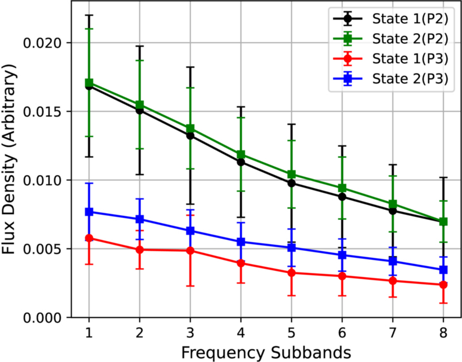
Figure 9. from Wei Li et al 2026 Astrophys. J. Lett. 1008 doi:10.3847/2041-8213/ae986e https://dx.doi.org/10.3847/2041-8213/ae986e © 2026. The Author(s). Published by the American Astronomical Society.
