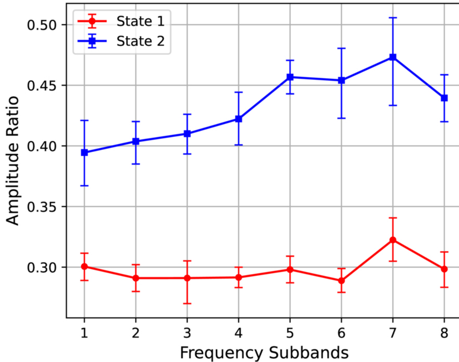
Figure 8. from Wei Li et al 2026 Astrophys. J. Lett. 1008 doi:10.3847/2041-8213/ae986e https://dx.doi.org/10.3847/2041-8213/ae986e © 2026. The Author(s). Published by the American Astronomical Society.
