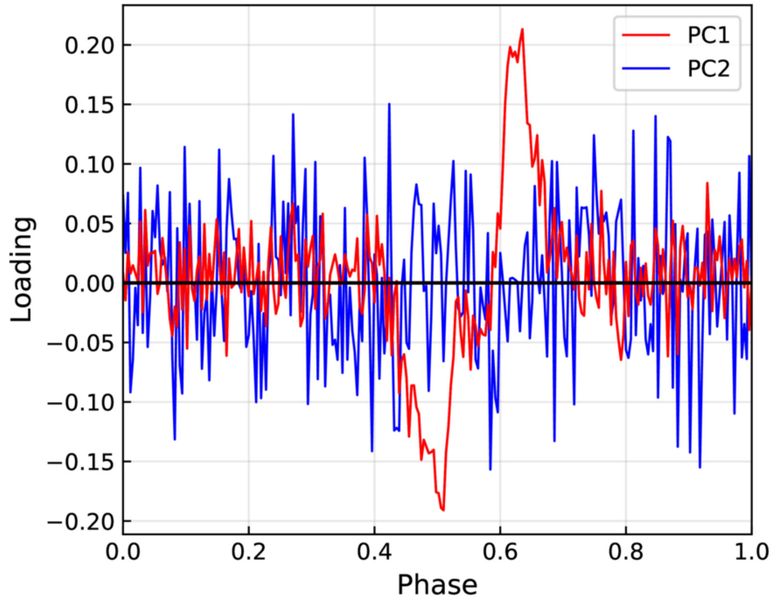
Figure 5. from Wei Li et al 2026 Astrophys. J. Lett. 1008 doi:10.3847/2041-8213/ae986e https://dx.doi.org/10.3847/2041-8213/ae986e © 2026. The Author(s). Published by the American Astronomical Society.
