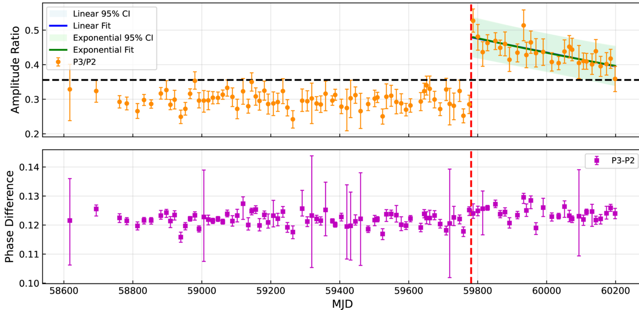
Figure 3. from Wei Li et al 2026 Astrophys. J. Lett. 1008 doi:10.3847/2041-8213/ae986e https://dx.doi.org/10.3847/2041-8213/ae986e © 2026. The Author(s). Published by the American Astronomical Society.
