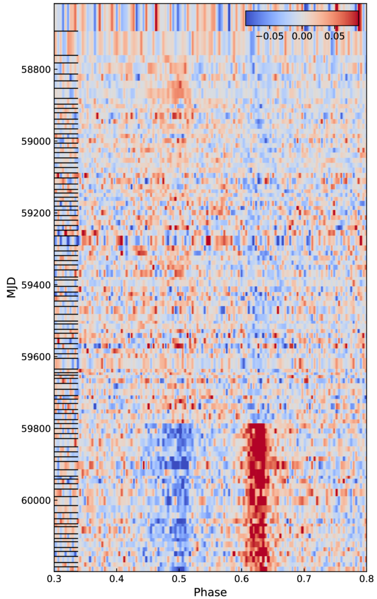
Figure 2. from Wei Li et al 2026 Astrophys. J. Lett. 1008 doi:10.3847/2041-8213/ae986e https://dx.doi.org/10.3847/2041-8213/ae986e © 2026. The Author(s). Published by the American Astronomical Society.
