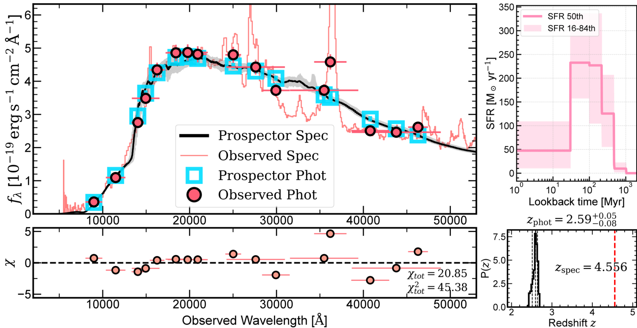
Figure A2. from Mingyu Li et al 2026 Astrophys. J. Lett. 1008 doi:10.3847/2041-8213/ae9863 https://dx.doi.org/10.3847/2041-8213/ae9863 © 2026. The Author(s). Published by the American Astronomical Society.
