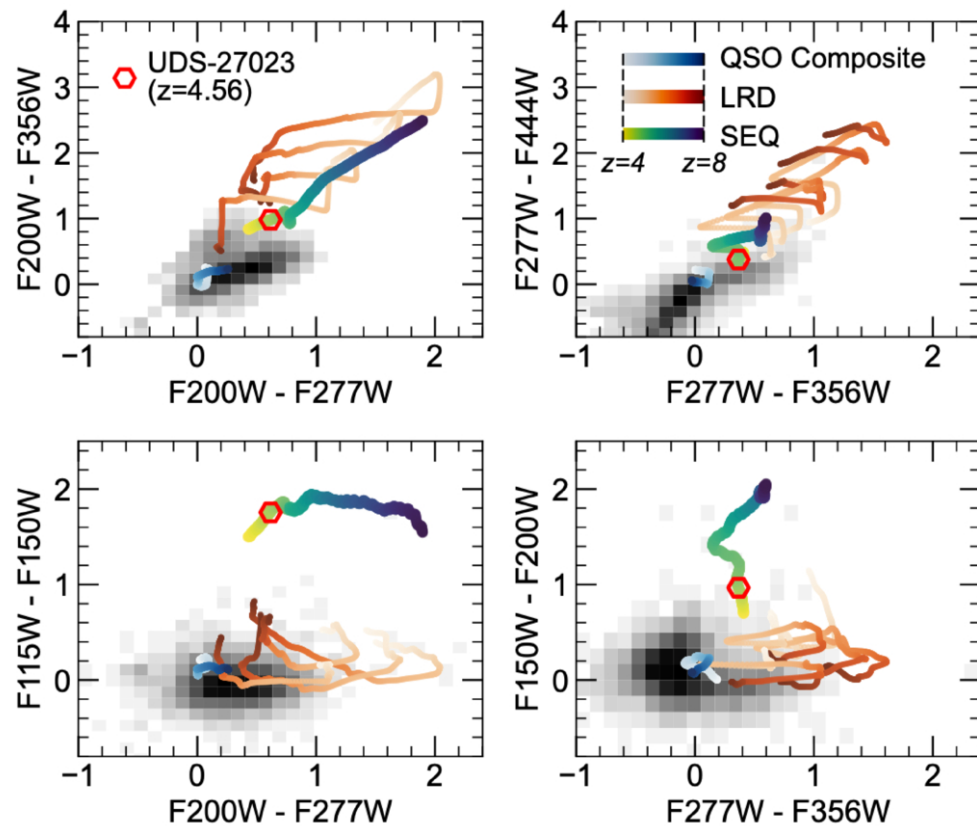
Figure A1. from Mingyu Li et al 2026 Astrophys. J. Lett. 1008 doi:10.3847/2041-8213/ae9863 https://dx.doi.org/10.3847/2041-8213/ae9863 © 2026. The Author(s). Published by the American Astronomical Society.
