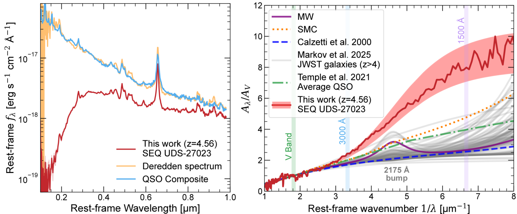
Figure 2. from Mingyu Li et al 2026 Astrophys. J. Lett. 1008 doi:10.3847/2041-8213/ae9863 https://dx.doi.org/10.3847/2041-8213/ae9863 © 2026. The Author(s). Published by the American Astronomical Society.
