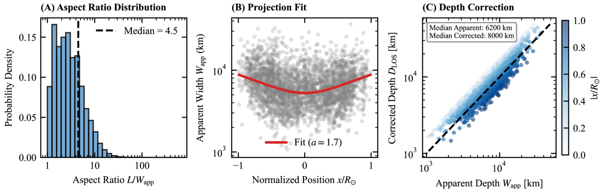
Figure 3. from T. Y. Xie et al 2026 Astrophys. J. Lett. 1008 doi:10.3847/2041-8213/ae9850 https://dx.doi.org/10.3847/2041-8213/ae9850 © 2026. The Author(s). Published by the American Astronomical Society.
