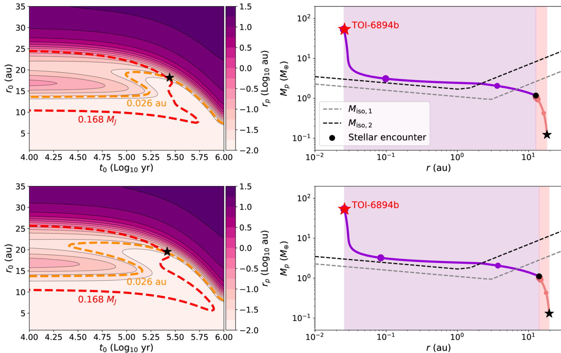
Figure 4. from Shunjing Zhao et al 2026 Astrophys. J. Lett. 1008 doi:10.3847/2041-8213/ae984f https://dx.doi.org/10.3847/2041-8213/ae984f
