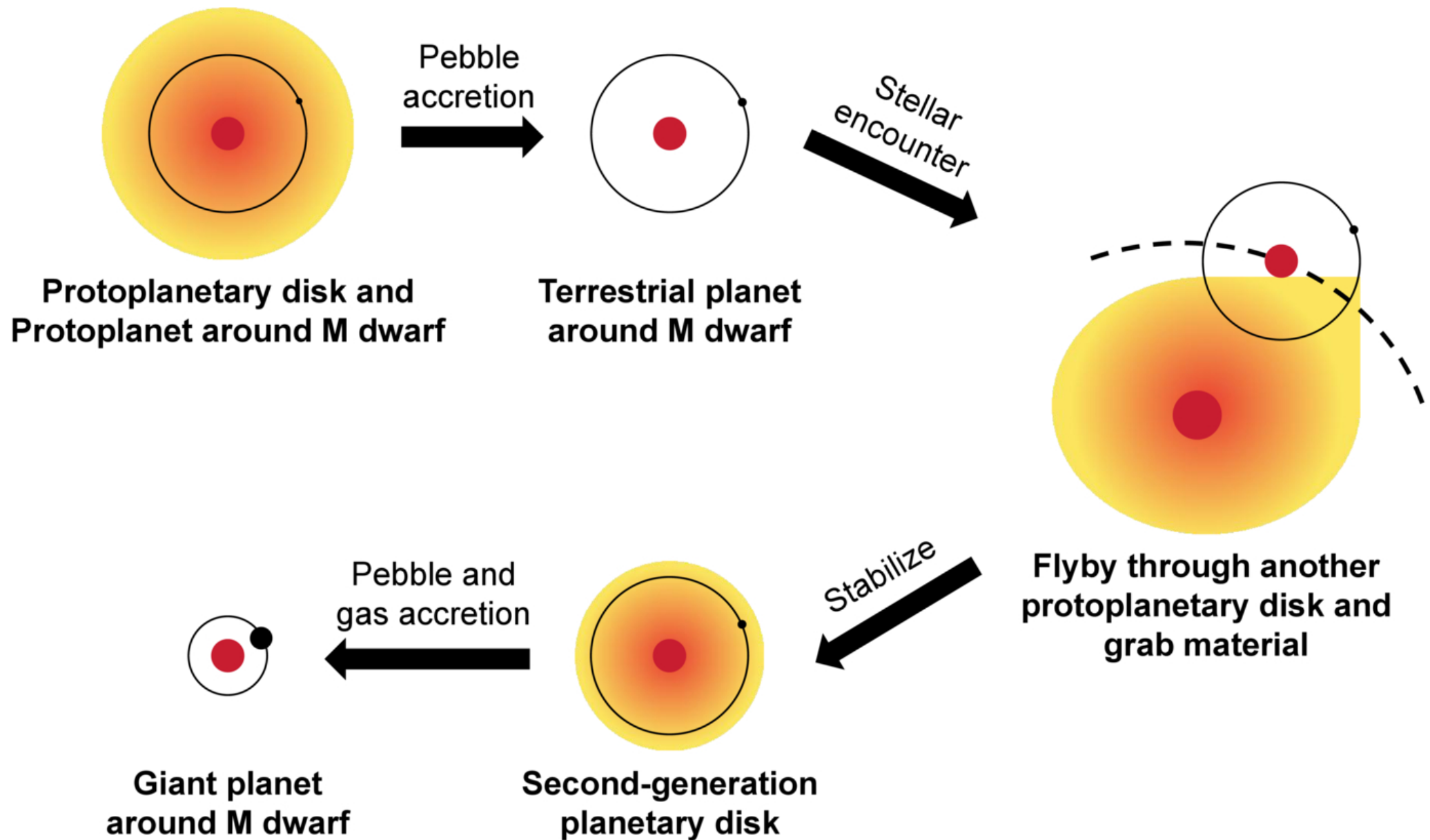
Figure 1. from Shunjing Zhao et al 2026 Astrophys. J. Lett. 1008 doi:10.3847/2041-8213/ae984f https://dx.doi.org/10.3847/2041-8213/ae984f © 2026. The Author(s). Published by the American Astronomical Society.
