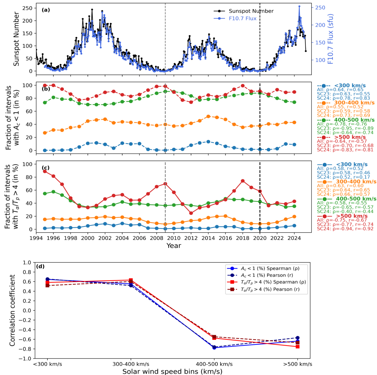
Figure 4. from Aakash Gupta et al 2026 Astrophys. J. Lett. 1008 doi:10.3847/2041-8213/ae984e https://dx.doi.org/10.3847/2041-8213/ae984e © 2026. The Author(s). Published by the American Astronomical Society.
