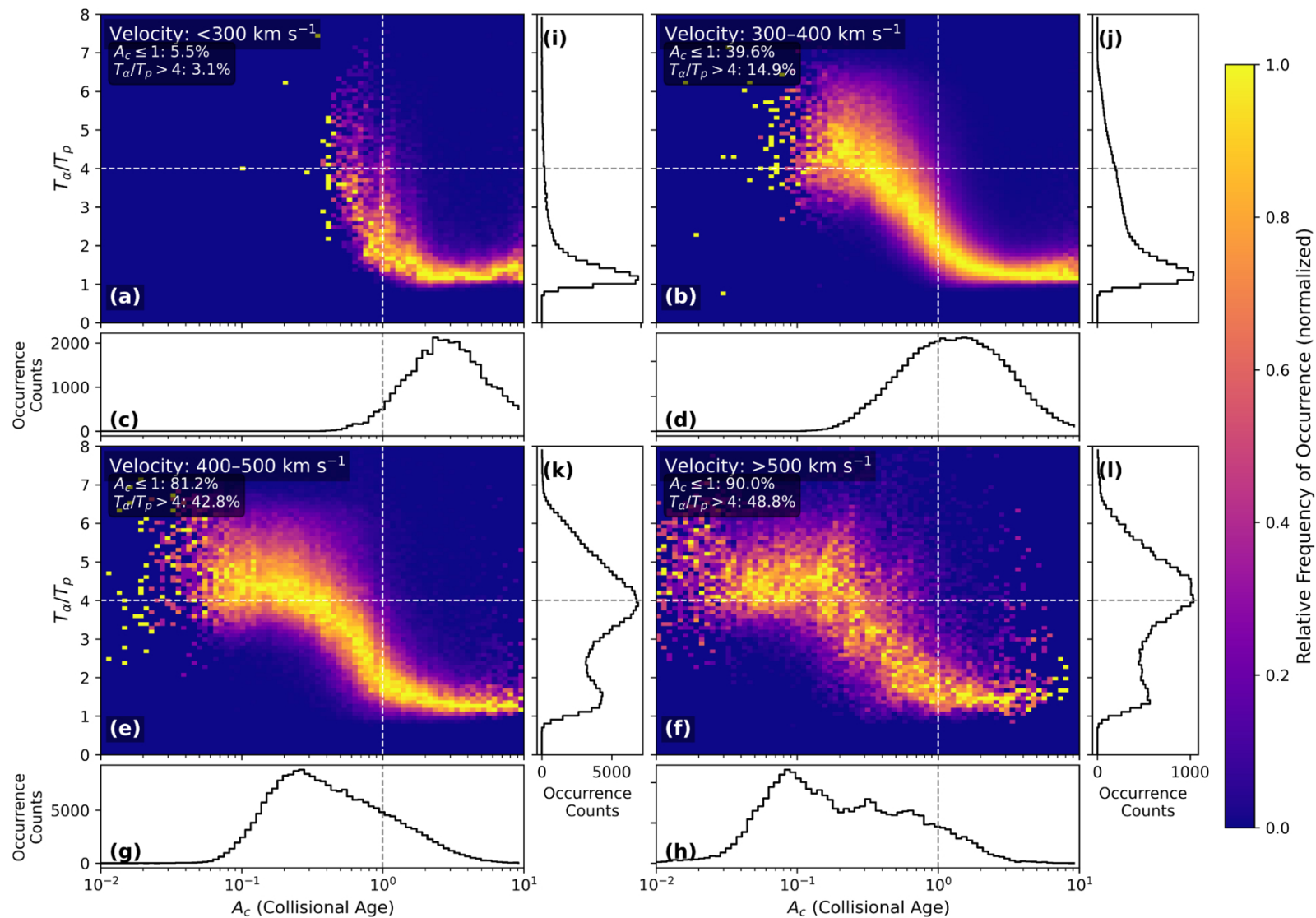
T_a/T_p vs Collisional Age with A_c Distributions
