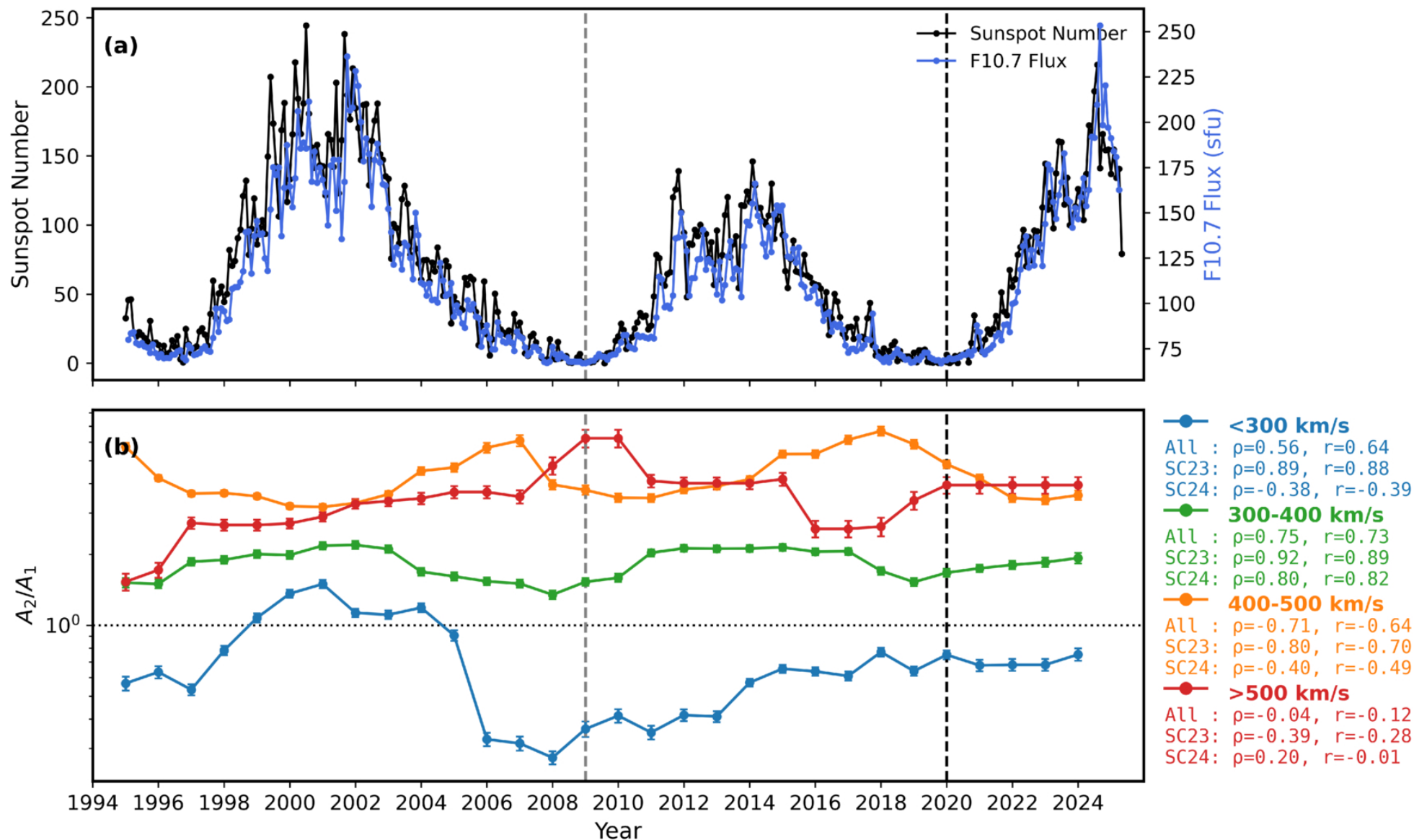
Figure 2. from Aakash Gupta et al 2026 Astrophys. J. Lett. 1008 doi:10.3847/2041-8213/ae984e https://dx.doi.org/10.3847/2041-8213/ae984e © 2026. The Author(s). Published by the American Astronomical Society.
