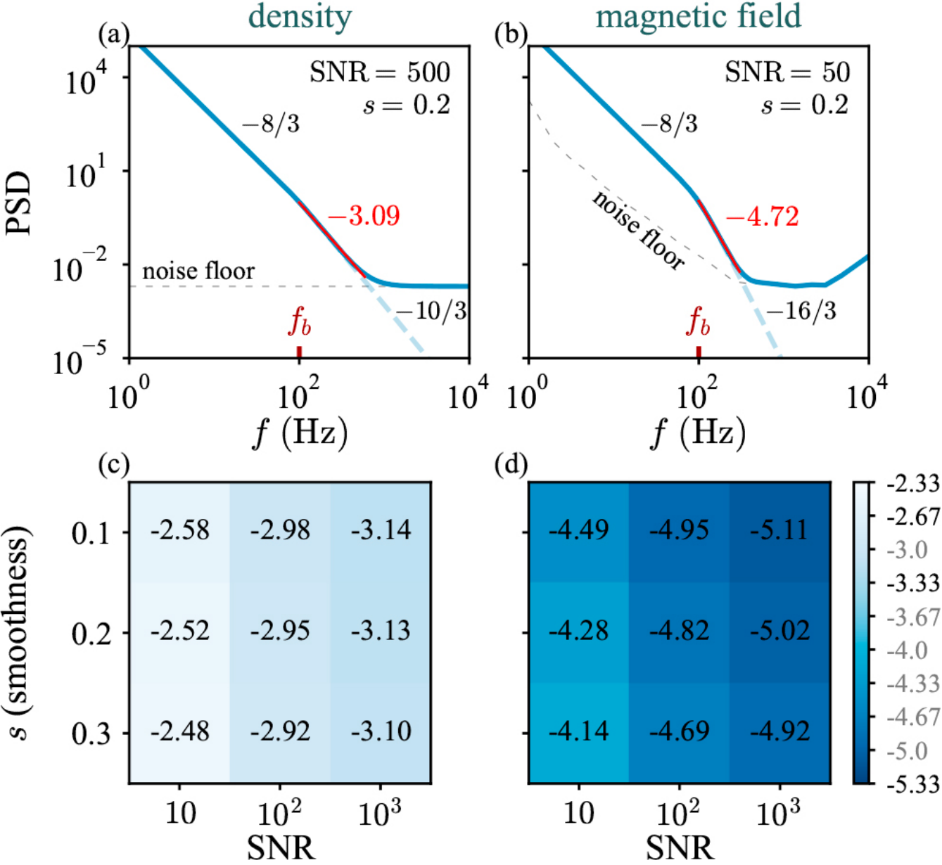
Figure 5. from Shiladitya Mondal et al 2026 Astrophys. J. Lett. 1008 doi:10.3847/2041-8213/ae984a https://dx.doi.org/10.3847/2041-8213/ae984a © 2026. The Author(s). Published by the American Astronomical Society.
