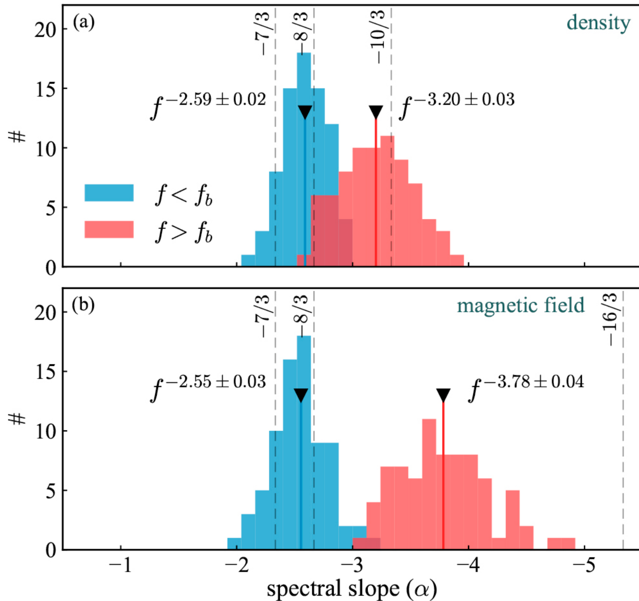
Figure 3. from Shiladitya Mondal et al 2026 Astrophys. J. Lett. 1008 doi:10.3847/2041-8213/ae984a https://dx.doi.org/10.3847/2041-8213/ae984a © 2026. The Author(s). Published by the American Astronomical Society.
