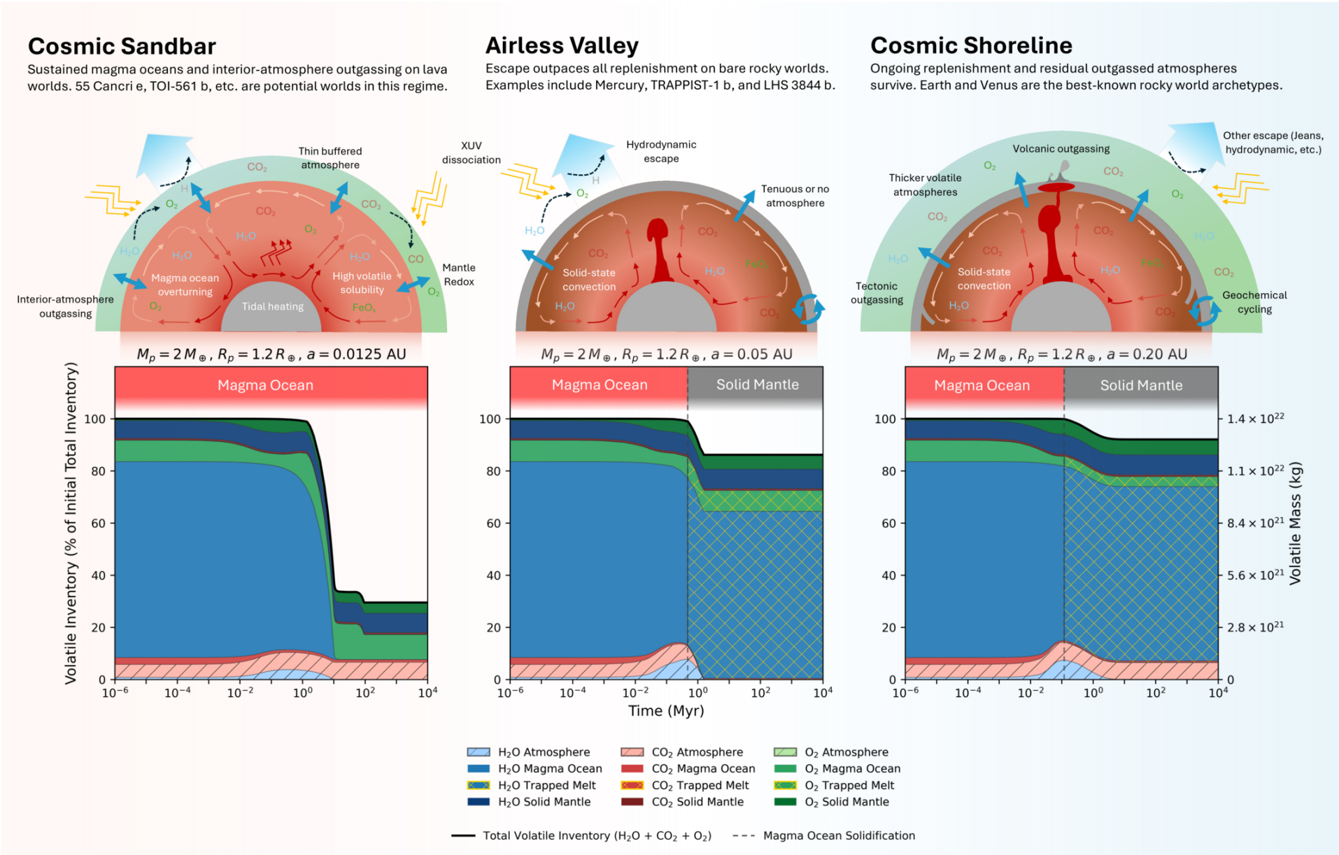
Figure 1. from Barron K. Nguyen et al 2026 Astrophys. J. Lett. 1008 doi:10.3847/2041-8213/ae9743 https://dx.doi.org/10.3847/2041-8213/ae9743 © 2026. The Author(s). Published by the American Astronomical Society.
