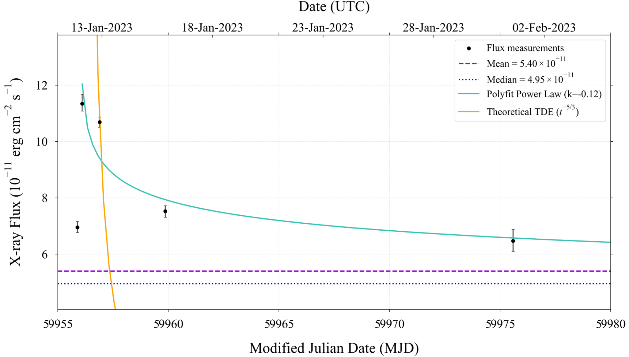
Figure 5. from Sarah Ketchum et al 2026 Astrophys. J. Lett. 1008 doi:10.3847/2041-8213/ae9742 https://dx.doi.org/10.3847/2041-8213/ae9742 © 2026. The Author(s). Published by the American Astronomical Society.
