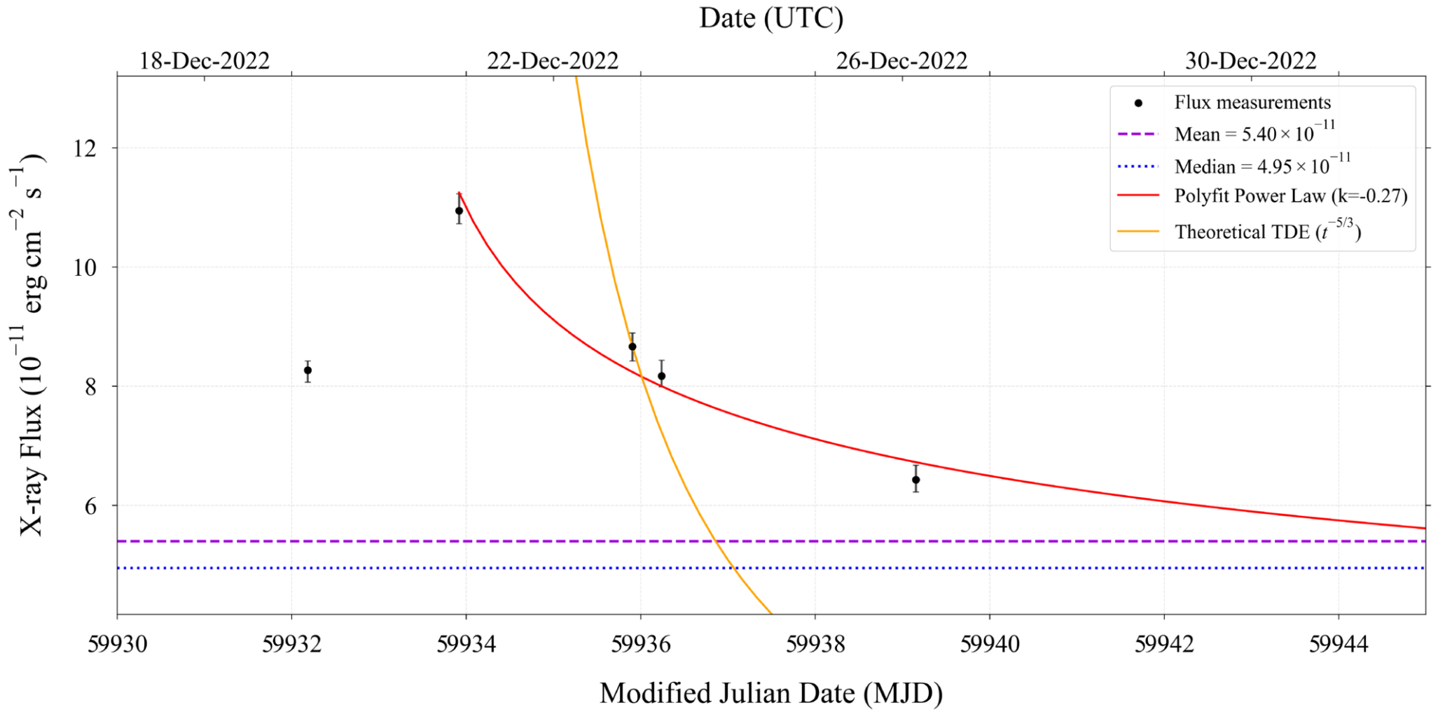
Figure 4. from Sarah Ketchum et al 2026 Astrophys. J. Lett. 1008 doi:10.3847/2041-8213/ae9742 https://dx.doi.org/10.3847/2041-8213/ae9742 © 2026. The Author(s). Published by the American Astronomical Society.
