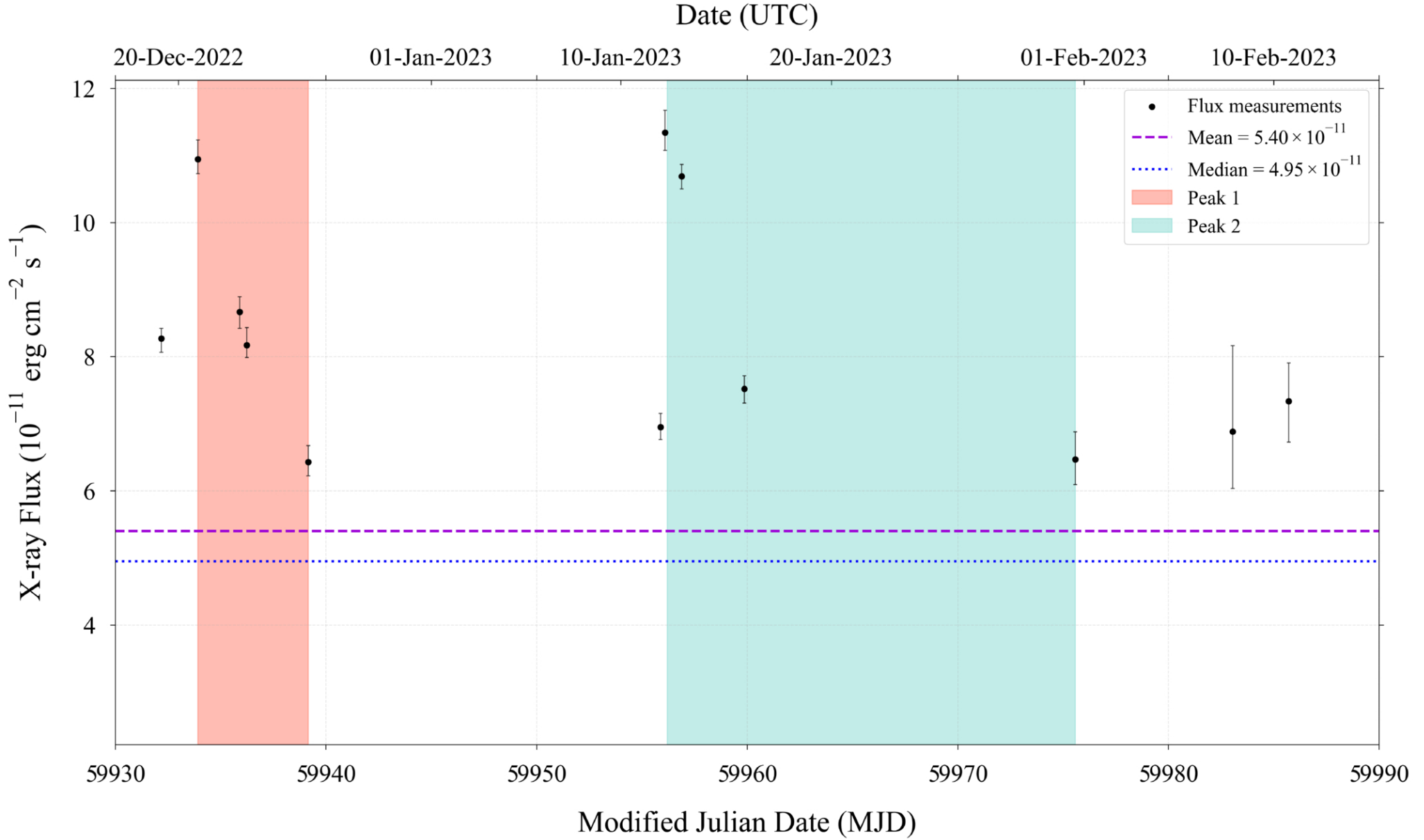
Figure 3. from Sarah Ketchum et al 2026 Astrophys. J. Lett. 1008 doi:10.3847/2041-8213/ae9742 https://dx.doi.org/10.3847/2041-8213/ae9742 © 2026. The Author(s). Published by the American Astronomical Society.
