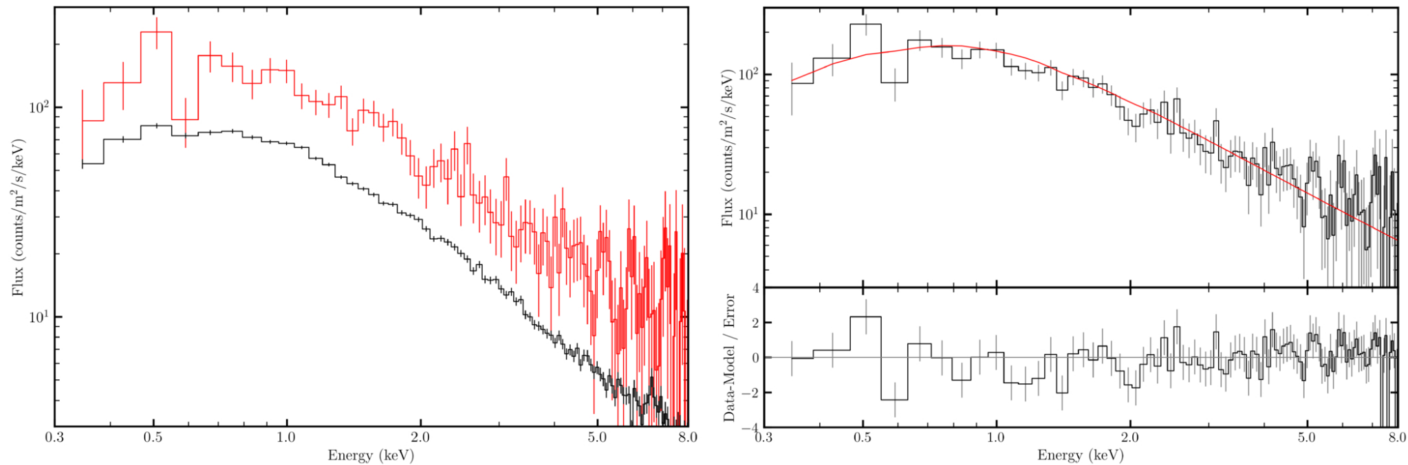
Figure 2. from Sarah Ketchum et al 2026 Astrophys. J. Lett. 1008 doi:10.3847/2041-8213/ae9742 https://dx.doi.org/10.3847/2041-8213/ae9742 © 2026. The Author(s). Published by the American Astronomical Society.
